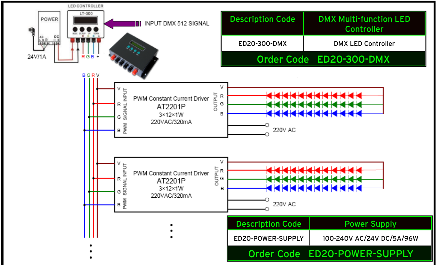
Schematic of multi function LED Controller and 3 x 12 1W RGB Floodlights
